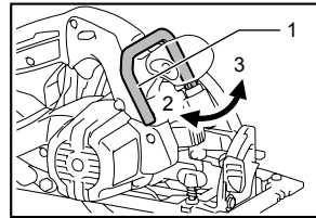
1. Hook 2. Close 3. Open
