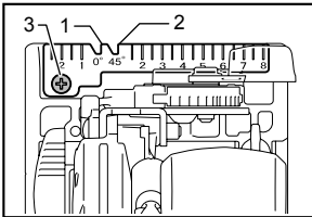
1. Cutting line ( 0^{\circ} position) 2. Cutting line ( 45^{\circ} position) 3. Screw
